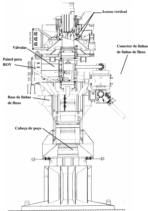
Figura A.3 - ANM-GLL ( guidelineless )
