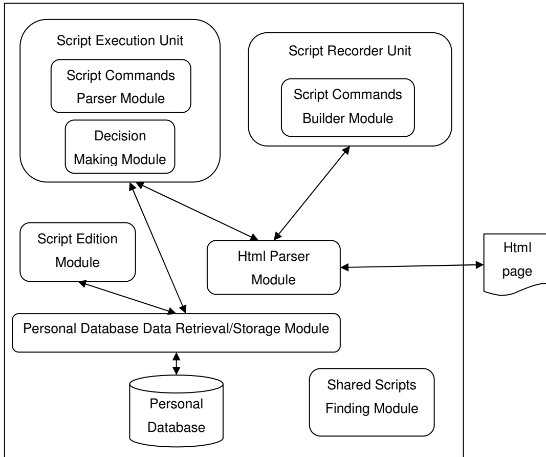
Figure 5: CoScripter Architecture
