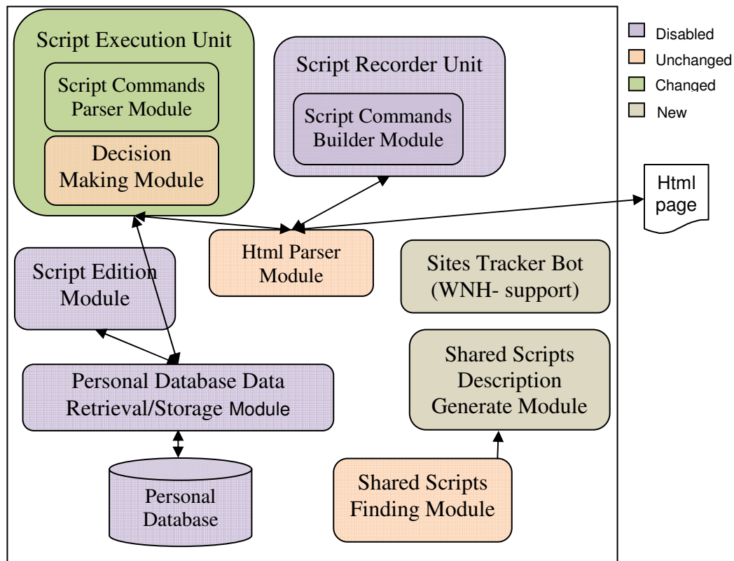
Figure 6: WNH Architecture
