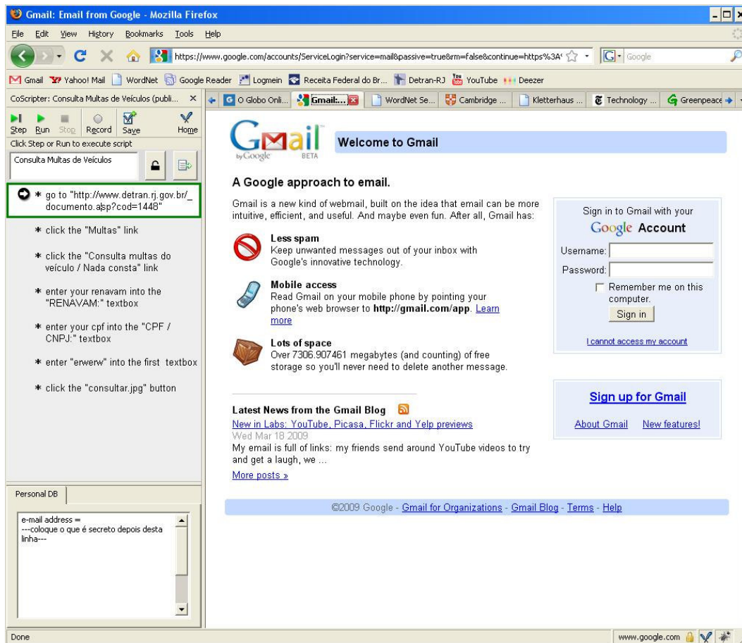
Figure 2: CoScripter
