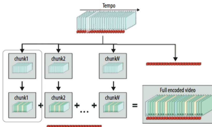
Figure 2.2. Split and Merge architecture. The system fragments every video received,
