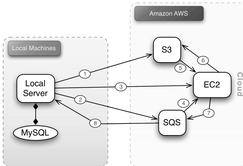
Figure 3.1. Architecture for the public submission system.
