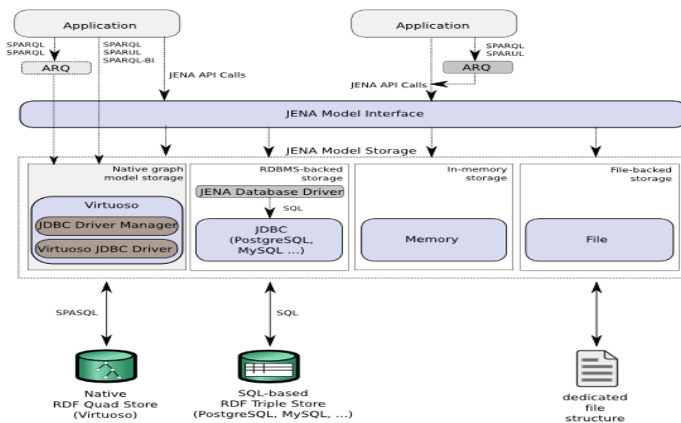
Figure 8 - Architecture of Virtuoso Jena Provider (Virtuoso 2012a)
