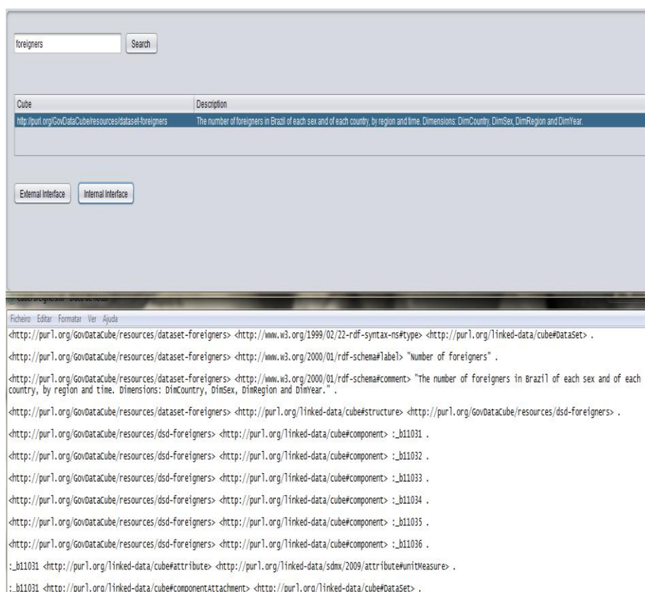
Figure 12 - Output of External Interface for the cube selected
