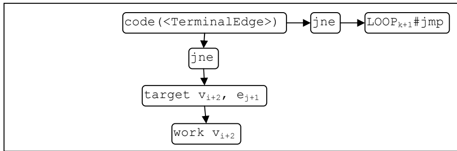
Figure 18 Terminal Edge code snippet
