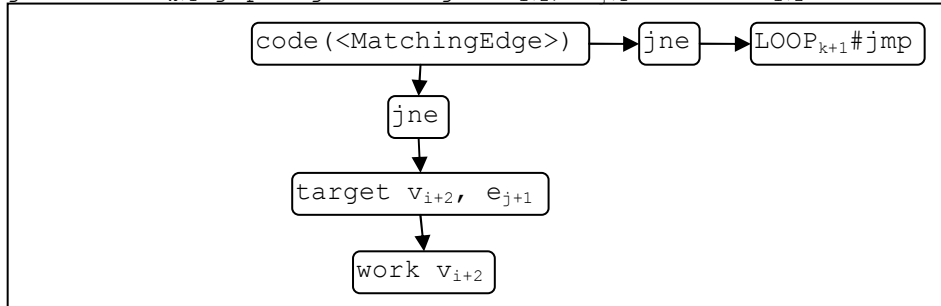
Figure 14 Matching Edge code snippet
