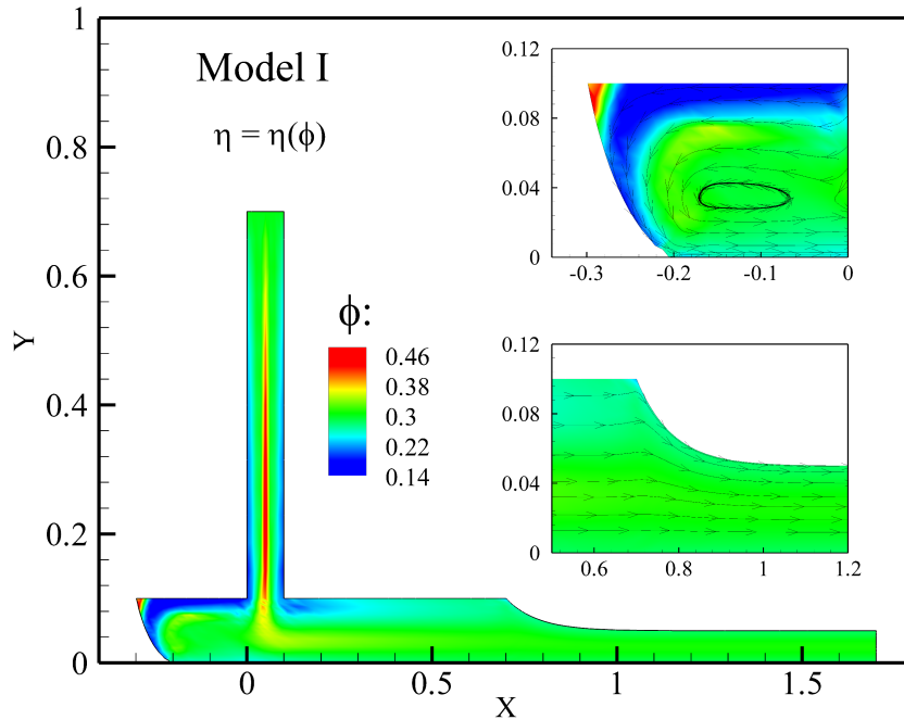
Figure 4.10: Contour map of particle concentration of the upstream region considering migration Model I and the viscosity model of Krieger.
