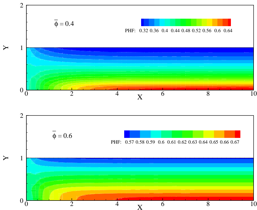
Figure 4.4: Countours for bulk concentrations 0.40 and 0.60, respectively.
