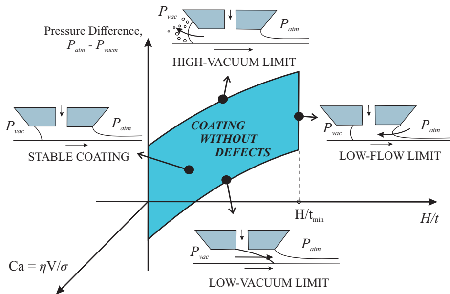
Figure 4.28: Coating window of a slot coating process as a function of the pressure difference ( P_{atm} - P_{vac} ), fixed Capillary number Ca and gap-top-thickness ratio H/t .
